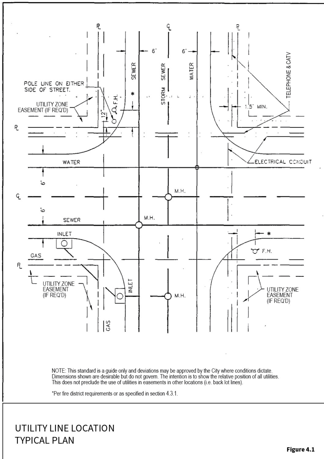
Figure 4-1. Utility Line Location: Typical Plan
