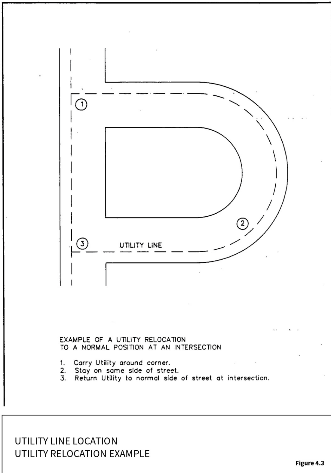
Figure 4-3. Utility Line Relocation Example
