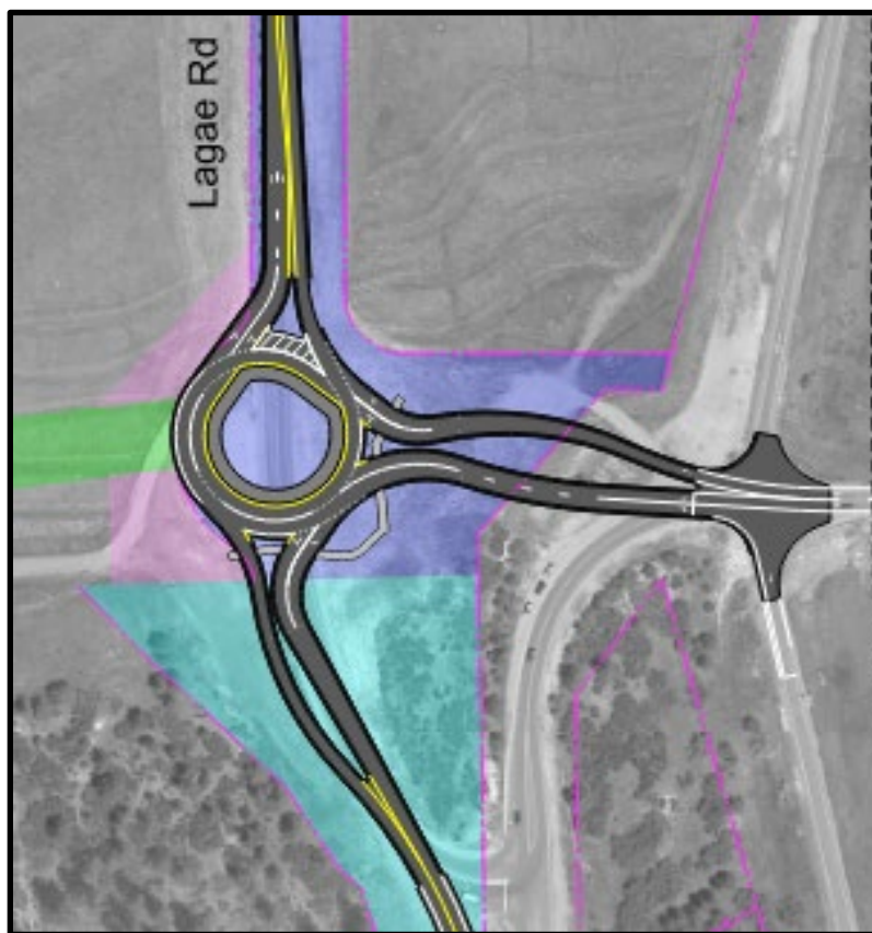
Figure 11. Lagae Road/Happy Canyon Road Intersection Improvements
