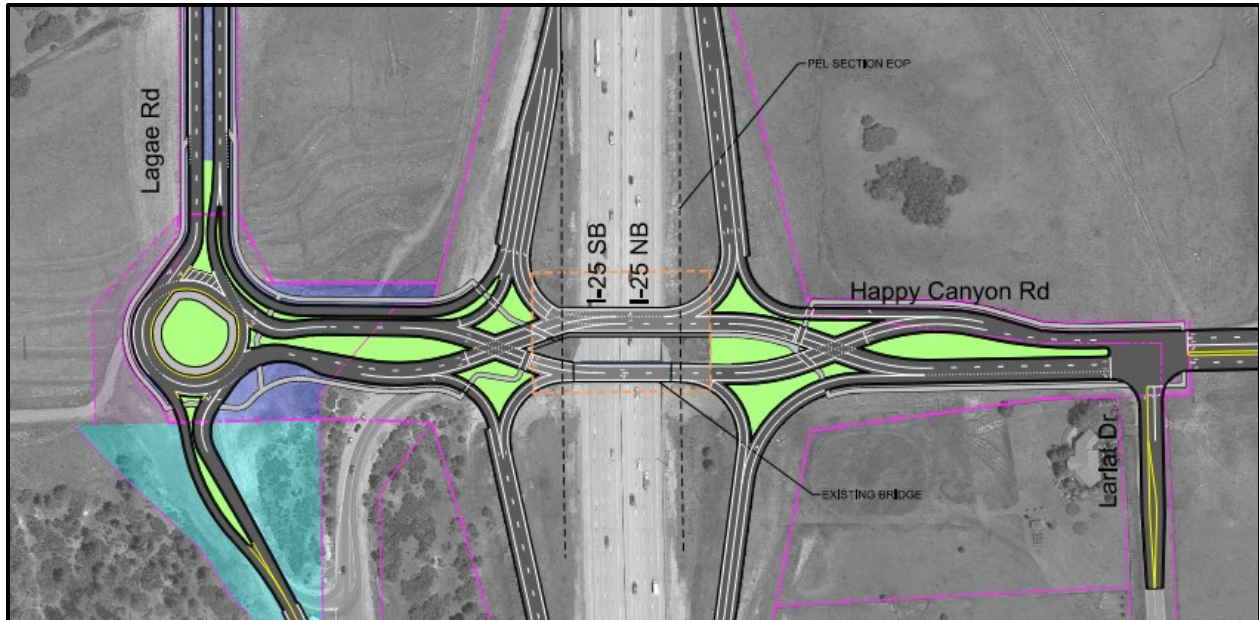
Figure 22. Diverging Diamond Interchange Alternative
