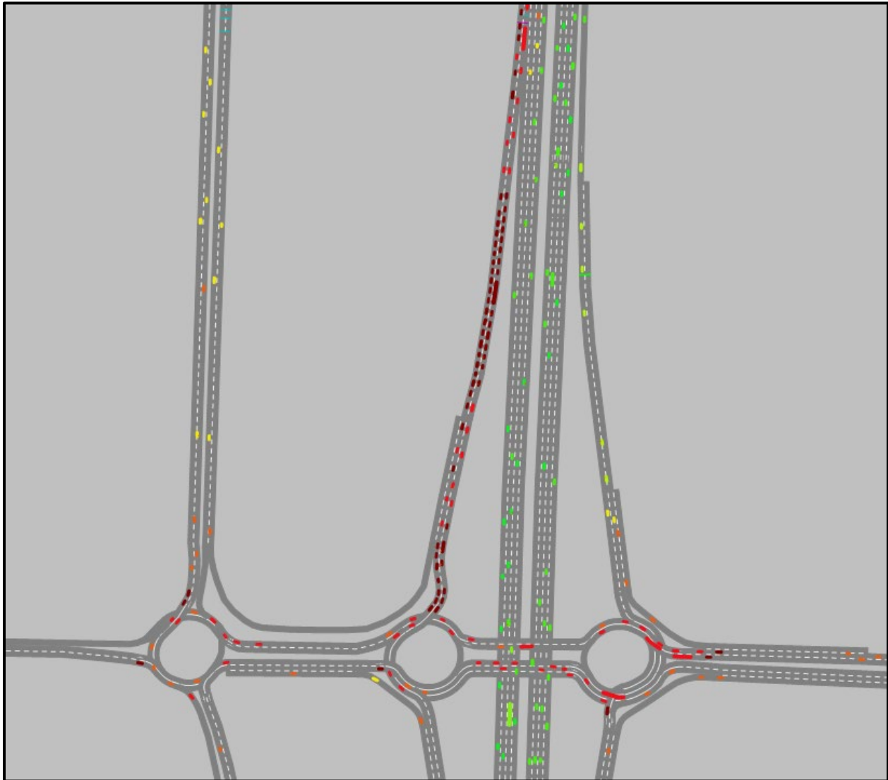
Figure 20. Roundabout Interchange Alternative Queuing (VISSIM)
