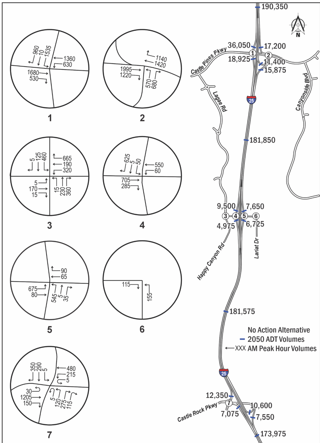
Figure 9. 2050 No Action AM Peak Hour Total Traffic Volumes
